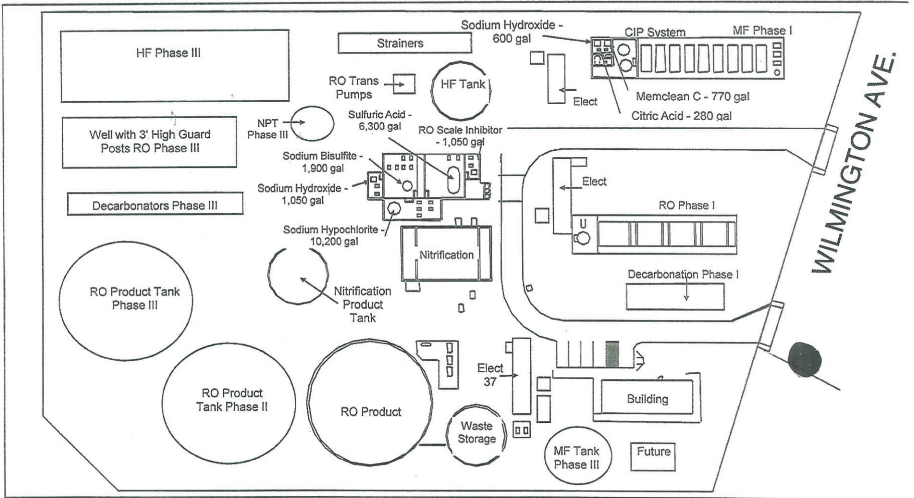
Carson Regional Water Recycling Plant
